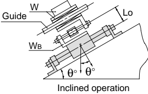
Inclined operation
