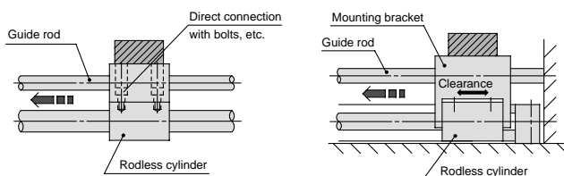
Figure 1. Incorrect mounting Variations in the load and cylinder shaft alignment cannot be assimilated, resulting in malfunction.
