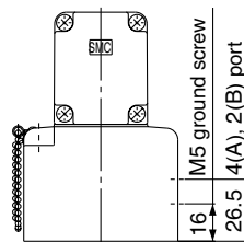
Bottom ported drawing
