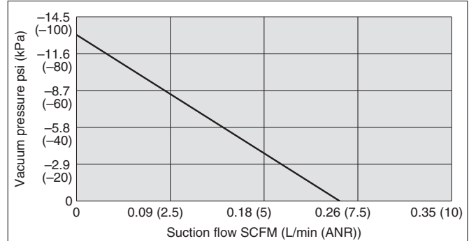
Flow-rate Characteristics
