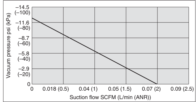
Flow-rate Characteristics
