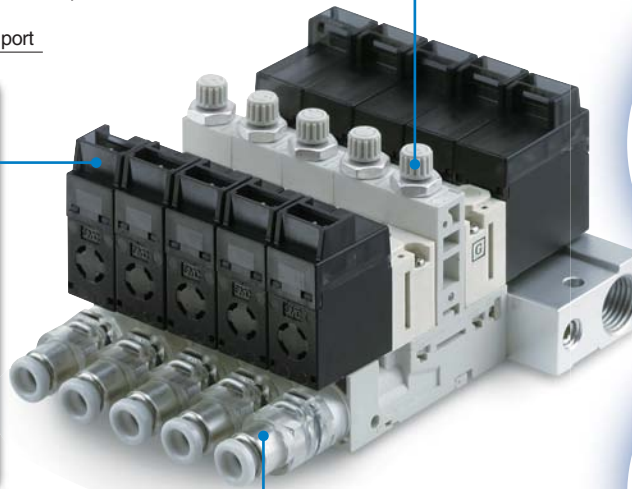
With pressure sensor
